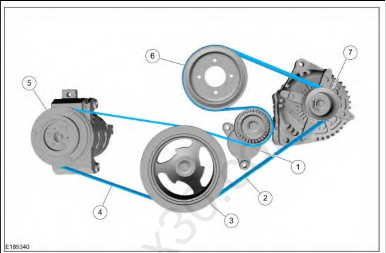
Fig 1: View Of Drive Belt And Pulley
